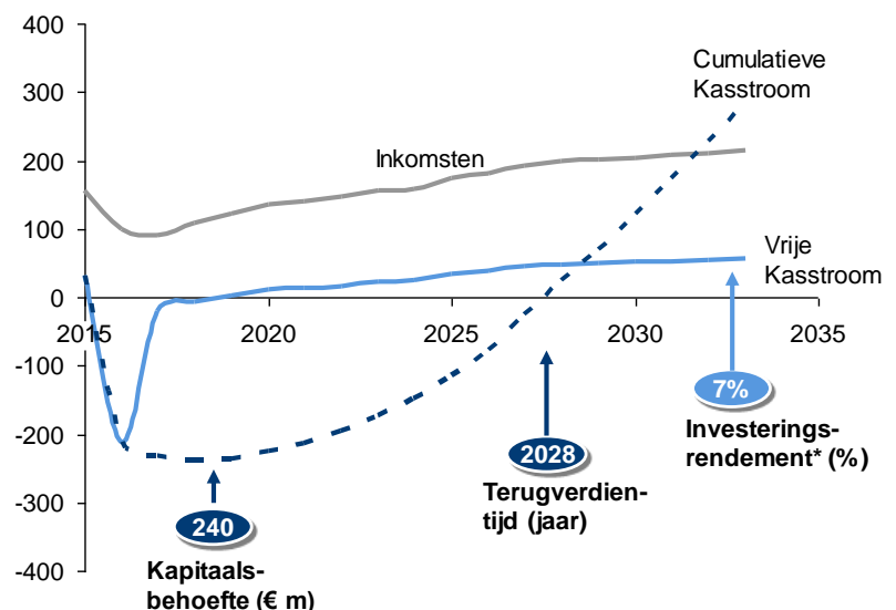
Kasstroom KCB in scenario, 2015-33 (€ m)
